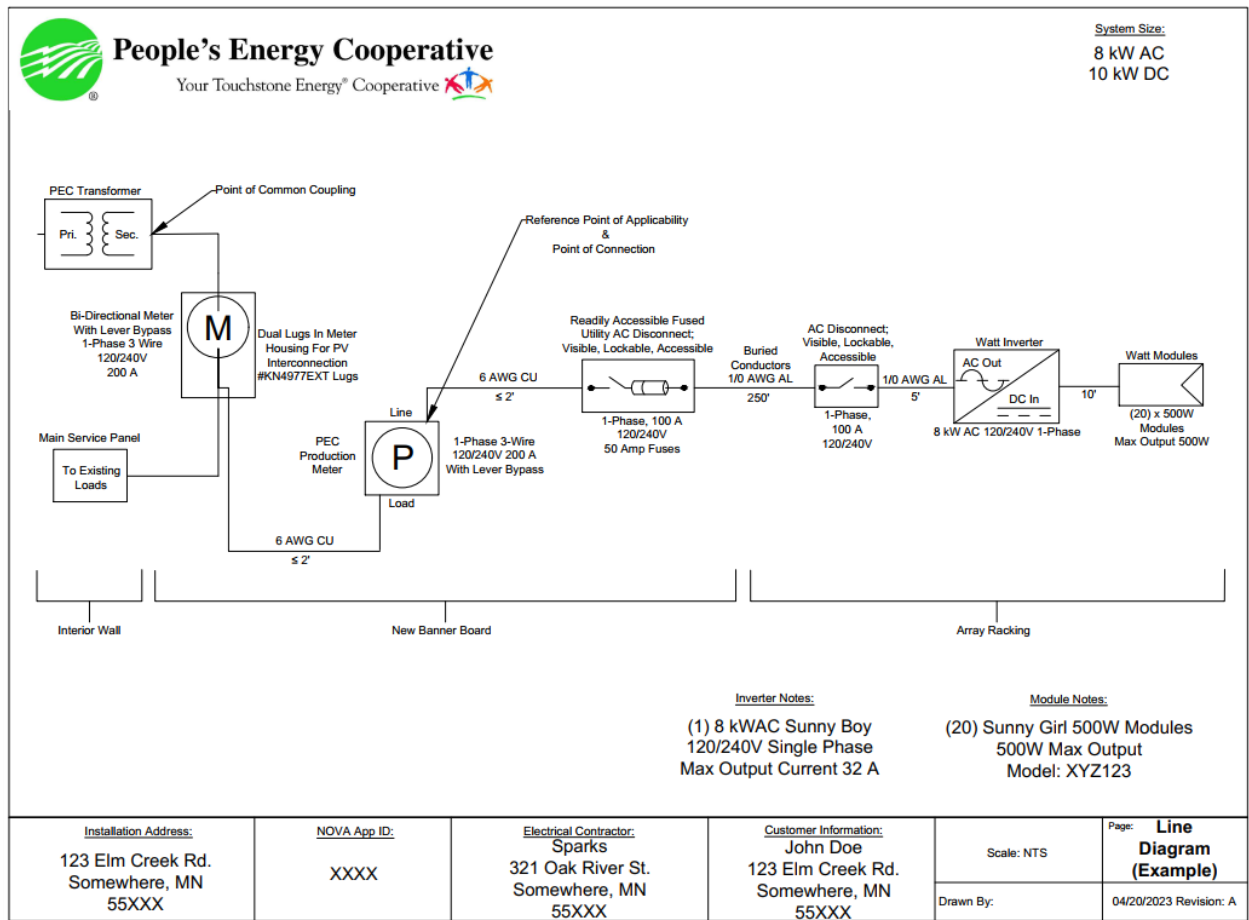
Figure 14.2 – Example Simplified One-Line Diagram
