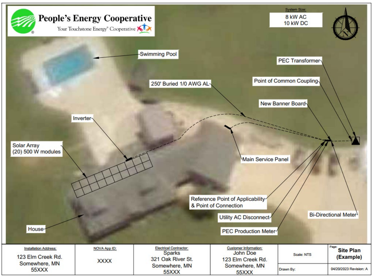
Figure 14.3 – Sample Simplified Site Diagram
