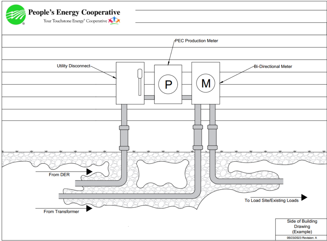
Figure 14.4b – Side of building equipment layout drawing:
