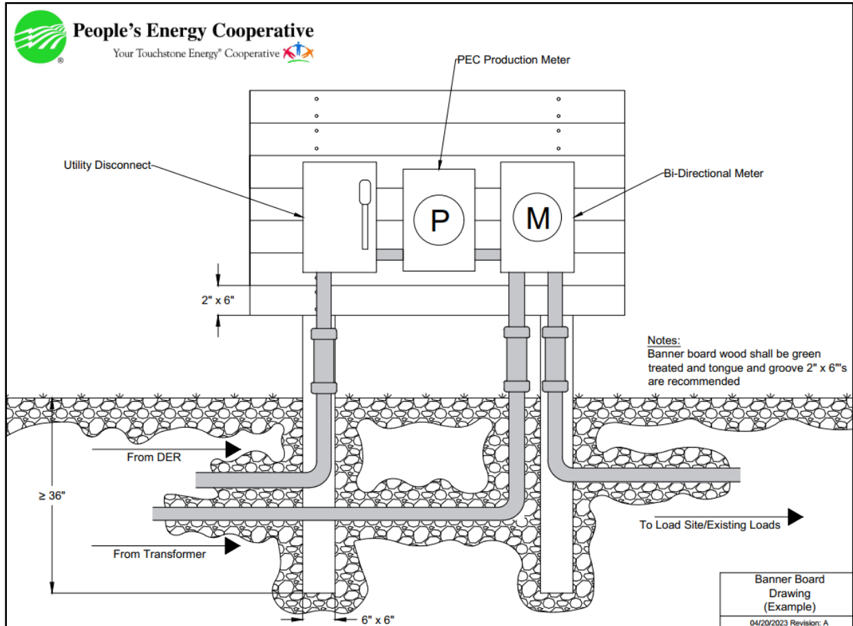
Figure 14.4a – Banner board equipment layout drawing:
